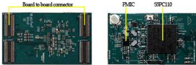
[CPU board]
